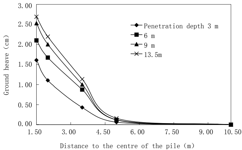
Figure 10 Distributions of the surface heave over the lateral distance from the centre of the casing for penetration depths of 3, 6, 9 and 13.5 m
