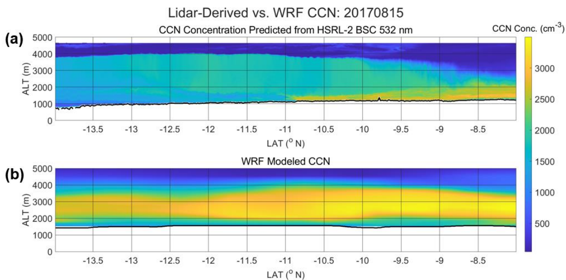
Figure 8: (a) Derived curtain of CCN concentrations from the HSRL-2 backscatter coefficient at 532 nm for an ORACLES P-3 track on 15 August 2017. The black line corresponds to HSRL-2 cloud top height altitudes. (b) WRF-CAM5 model CCN curtain corresponding to the same P-3 track. The black line corresponds to the nearest HSRL-2 -interpolated altitude at WRF-estimated cloud top height.
