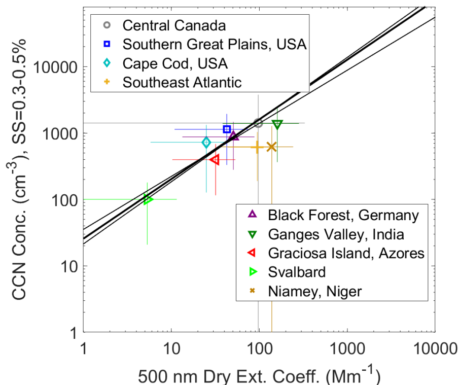
450 Figure 7: Adapted from Figure 6 in Shinozuka et al. (2015), campaign-average in situ CCN concentration and in situ dry extinction at 500 nm are overlaid, using the label "Southeast Atlantic." The error bars are calculated using standard deviation, and the original best fit lines have not been altered. The supersaturation (SS) for these observations ranges from 0.3-0.5% to match the analysis done in Shinozuka et al. (2015).
