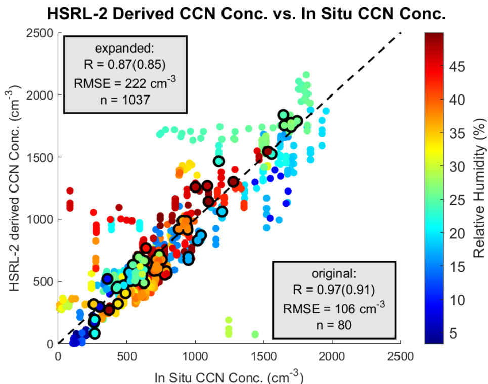
Figure 9: In situ CCN concentration vs. HSRL-2 derived CCN concentration is given for an expanded three year data set ( dt = \pm 0.5\text{hr} , dd = \pm 4.4\text{km} , dh = 45\text{m} ). The supersaturation in the expanded data set ranges from 0.15-0.4% and the supersaturation for the original collocated data set ranges from 0.22-0.4%. The points with a black outline designate those included in the original collocated data set that was used to develop the lidar-derived CCN concentration. The dashed line represents the 1:1 line, and for each data set the Pearson correlation coefficient is shown, with Spearman rank correlation coefficient given in parentheses. This comparison shows the general applicability of our regression equations to derive CCN concentrations using HSRL-2 observables over a larger subset of the ORACLES observations.
