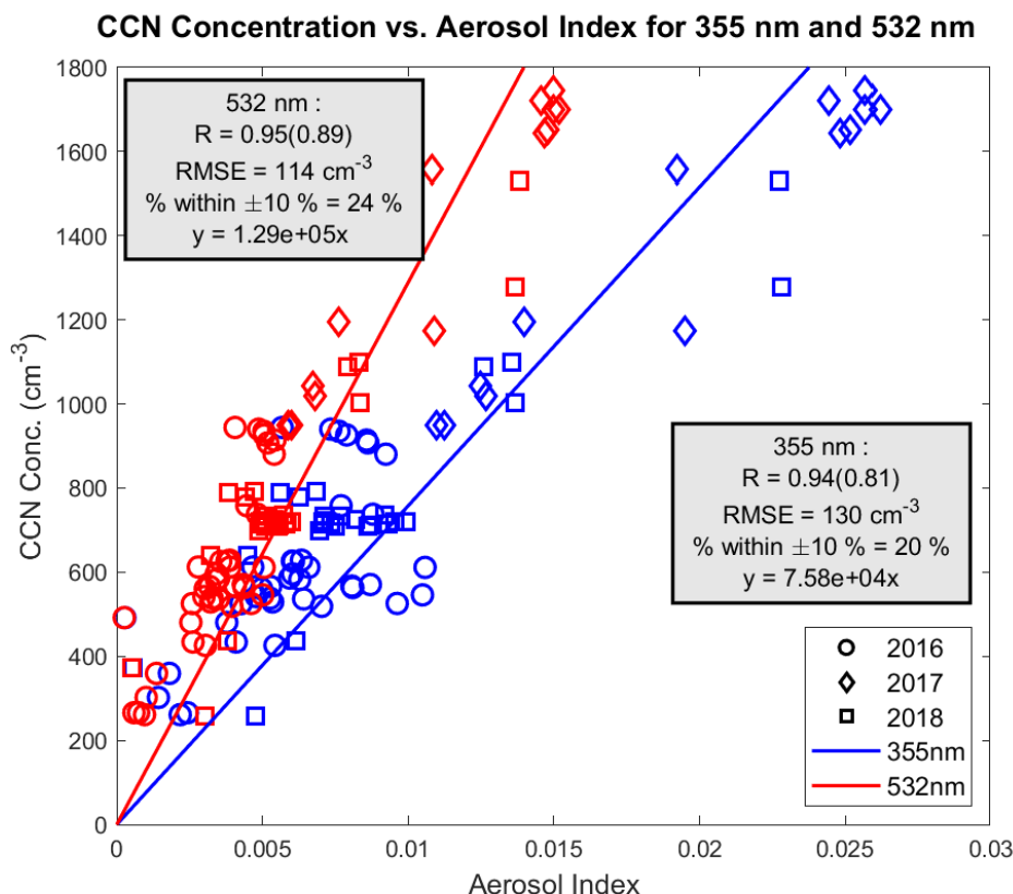
335 Figure 4: CCN concentration vs. aerosol index is given for the combined three year data set. Blue scatter points show results calculated using extinction at 355 nm and red scatter points show results calculated using extinction at 532 nm. Supersaturation for these observations ranges between 0.22-0.4%. Lines of best fit are forced through the origin to represent practicality of using linear regression equations to quantitatively obtain CCN concentrations using lidar observables. The Pearson correlation coefficient is shown, with Spearman rank correlation coefficient given in parentheses. 340
