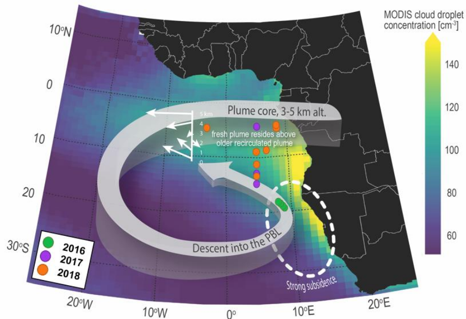
415 Figure 5: Adapted from Redemann et al., (2021), this schematic shows the commonly occurring trajectory of smoke aerosols ejected over the Southeast Atlantic. Overlaid are approximate locations of collocated observations from 2016 (green), 2017 (purple), and 2018 (orange). By comparing their locations to the schematic, we hypothesize that the collocated observations made in 2016 are older aerosols, while collocated observations of aerosols in 2017 and 2018 are likely fresher and more recently ejected from the smoke plume.
