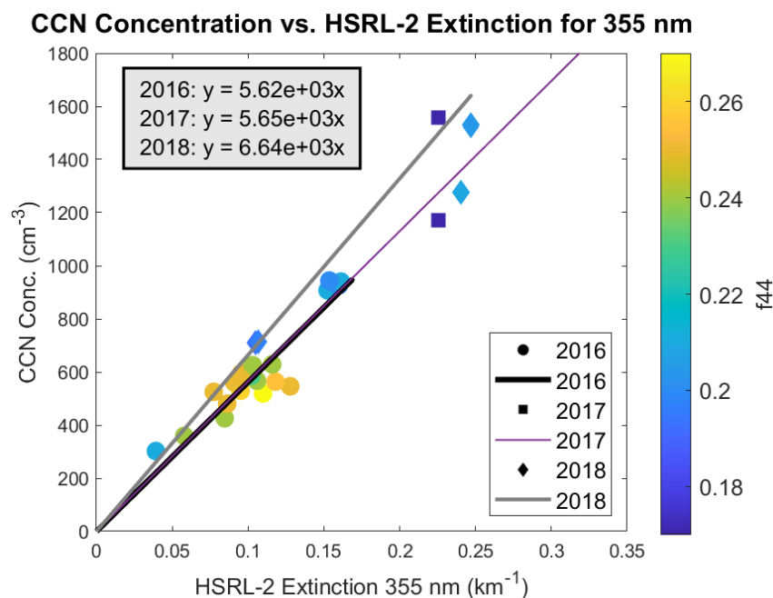
420 Figure 6: CCN concentration vs. HSRL-2 extinction coefficient at 355 nm for 2016 (circles), 2017 (squares), and 2018 (diamonds) collocated data sets. Supersaturation for these observations ranges between 0.22-0.4%. The scatter points are color-coded by f_{44} value. The f_{44} values range from 0.2-0.27 for 2016, 0.17 for 2017, and 0.19-0.21 for 2018. The number of data points is lower than the full number of full collocated data points due to missing f_{44} data. Lines of best fit are forced through (0,0) to represent the practicality of using linear relationships to quantitatively obtain CCN concentrations from lidar observables.
