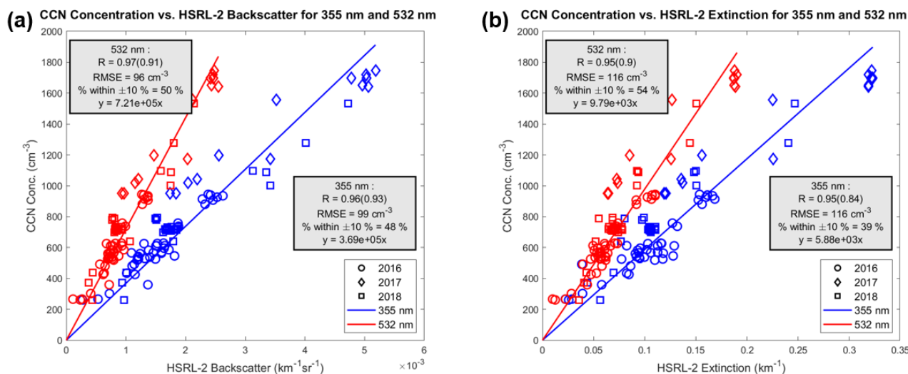
315 Figure 3: CCN concentration vs. HSRL-2 backscatter and extinction coefficients, with both wavelengths shown on each panel. This combined data set represents 10 days of observations and 80 total collocated data points (per coefficient), covering all three years of ORACLES. Supersaturation for these observations ranges between 0.22-0.4%. Lines of best fit are forced through the origin to represent practicality of using linear regression equations to quantitatively obtain CCN concentrations using HSRL-2 observables. The Pearson correlation coefficient is shown, with Spearman rank correlation coefficient given in parentheses.
