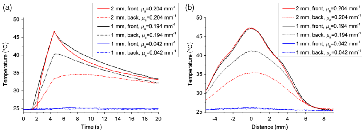
Fig. 7 (a) Temporal profiles for different phantoms, measured from front and backside and (b) spatial temperature profiles along Y -axis from Figs. 4 to 6 crossing temperature maximum, at the end of laser irradiation, after \sim 3 s of exposure. Measurements were conducted using laser parameters: T = 50 ms, \tau = 25 ms, N = 60 .
