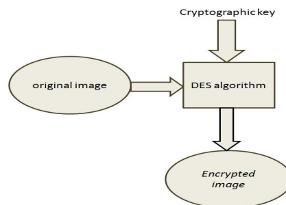
Figure 5.1: Encryption
