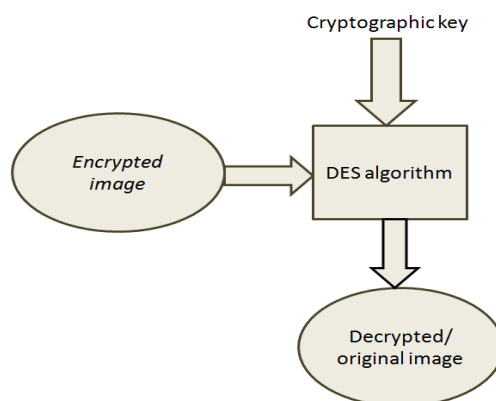
Figure 5.2: Decryption
