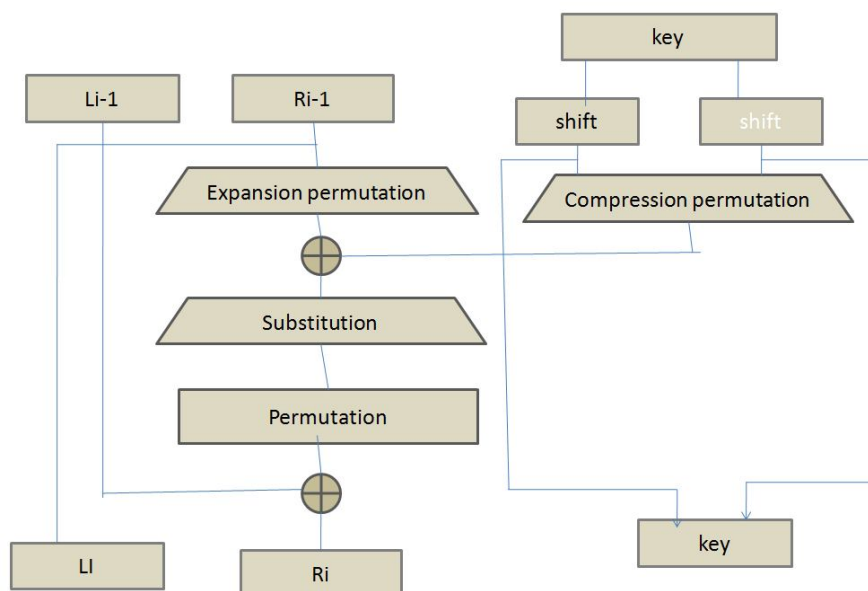
Figure 3.1: One round of DES
