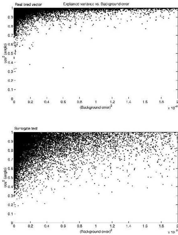
Fig. 11. Explained variance (square of the cosine of the angle between the background error and the space defined by the local vectors) as a function of the background error squared, computed for 90 days over every grid point. (a) using 10 bred vectors corresponding to the same time as the background error. (b) using 10 surrogate bred vectors corresponding to random times.
