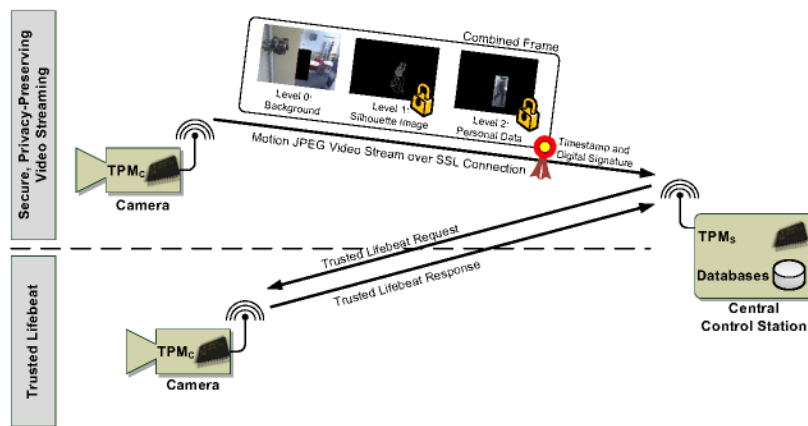
Fig. 3 From the central control station, the status of a camera can be reliably checked via a trusted lifebest. Secure video streaming ensures confidentiality, integrity, authenticity and freshness of image data. Furthermore, multi-level privacy protection and per-level access control are supported.
