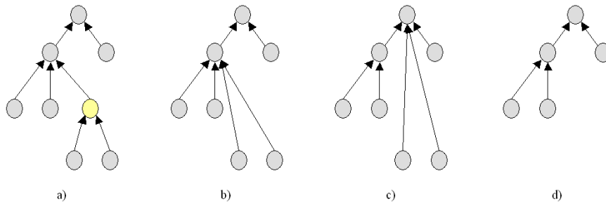
Figure 4. Resolution Points for Deleting Concept C: a) Original ontology; b) Connection to the parent concept; c) Connection to the root concept; d) Deletion of the subconcepts
