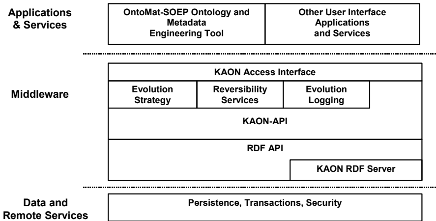
Figure 7. Conceptual KAON Architecture with Respect to Ontology Evolution
