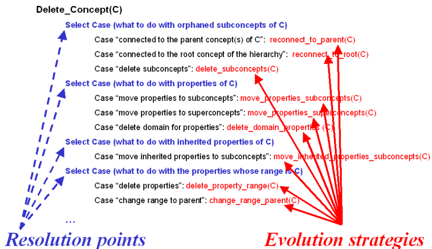
Figure 5. Part of algorithm for Concept Deletion, represented in the pseudo-code
