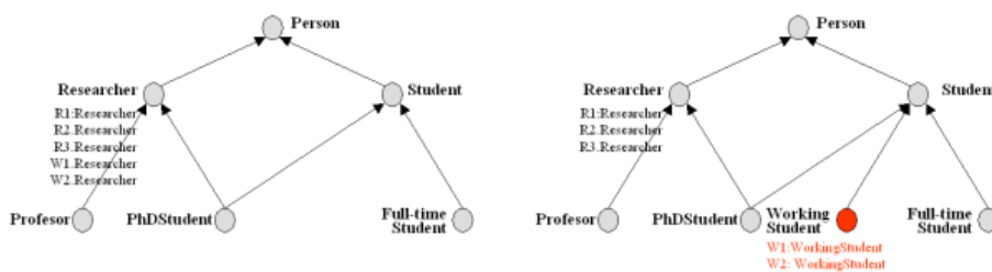
Figure 6. Instance-driven evolution strategy
