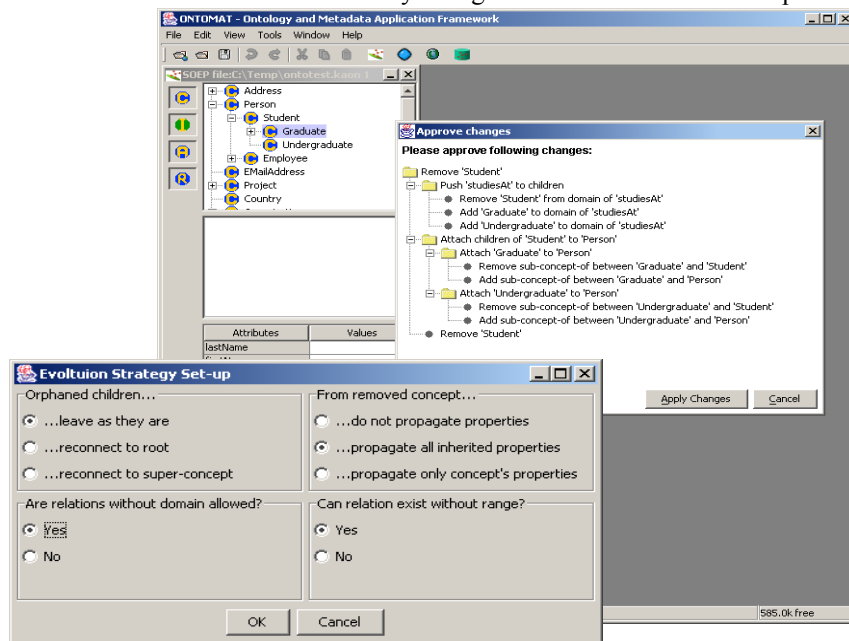
Figure 8. Ontology Evolution in KAON framework: Evolution Strategy Set-up and Ontology Evolution User Interface in OntoMat-SOEP
