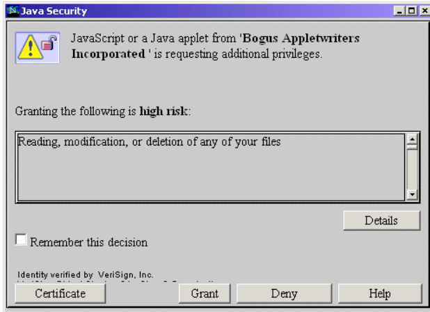
Figure 8. Applet requests a privilege by calling enablePrivilege("UniversalFileAccess") .
