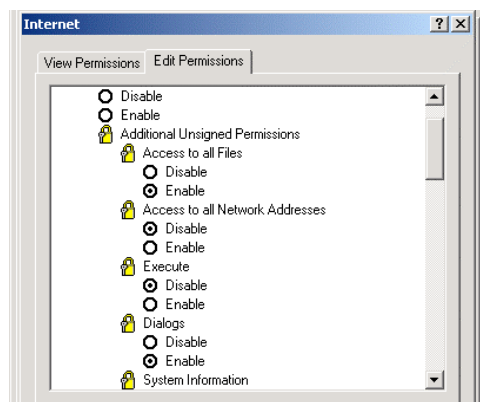
Figure 2. Java security settings in Internet Explorer.
