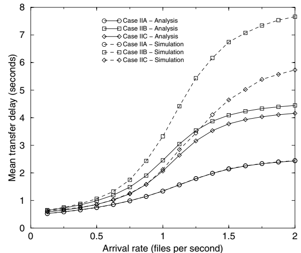
Fig. 4. Mean transfer delay for class-1 users as function of file arrival rate for Cases IIA-C
