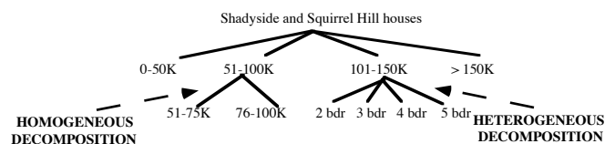
Figure 1: Aggregation: homogeneous & heterogeneous decomposition.
