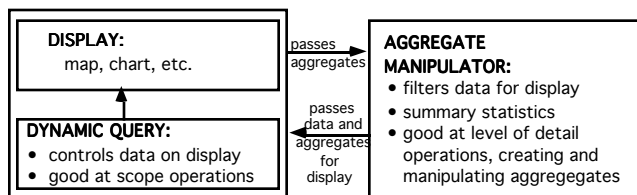
Figure 3: Data Flow for the AM & DQ.
