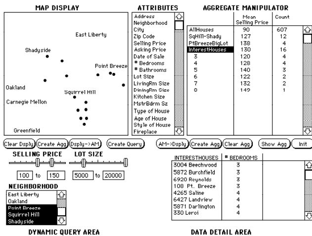
Figure 6: The workspaces of the interface: display, attributes, aggregate manipulator, data detail area and dynamic query area.
