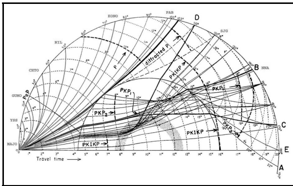
Figure 1: Schematic cross-section of the earth. Several ray paths of P-waves are displayed.
