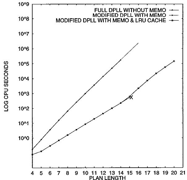
Figure 2: Full DPLL without memoization v. modified DPLL with memoization v. modified DPLL with memoization and LRU caching for SAND-CASTLE-67
