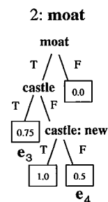
Figure 1: Sequential-Effects-Tree Representation For SAND-CASTLE-67
