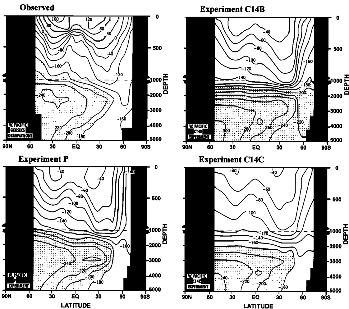
Figure 2. Western Pacific sections of \Delta^{14}\text{C} (per mil) in observations (top left) and in the natural radiocarbon experiments P, C14B, and C14C of Toggweiler et al. [1989a]. Experiments C14B and C14C are from two robust-diagnostic experiments (C14B treats vertical diffusion rates with a depth-dependent profile, whereas C14C adopts a constant vertical diffusivity). Experiment P is identical to experiment C14B, only there is no interior robust-diagnostic restoring of temperature-salinity (T-S).
