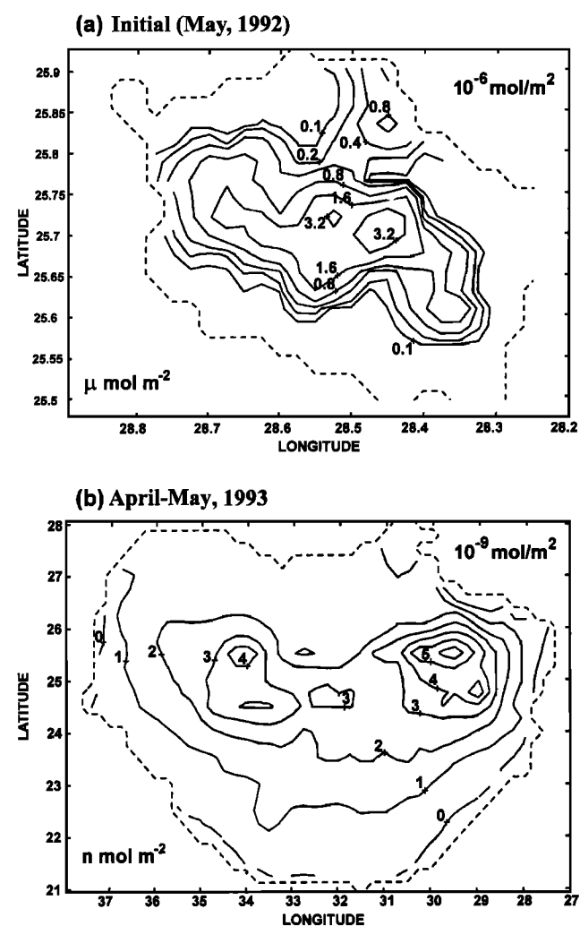
Figure 25. Map of the initial (May 1992) North Atlantic Tracer Release Experiment (NATRE) SF 6 tracer patch and that measured during April–May 1993 [from Ledwell et al. , 1998]. Note the different concentration and spatial scales in the two panels; the SF 6 tracer patch has spread from a highly concentrated 30- × 20-km zone in May 1992 to a more diluted 1000- × 1000-km region 1 year later.
