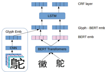
Figure 1: Architecture of our Glyph Models
