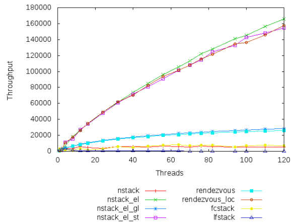
Figure 4: Results for 50% pushes and 50% pops
