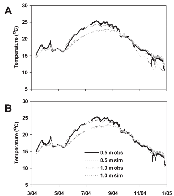
Fig. 13. Observed (obs) and simulated (sim) temperatures in the Merced River, CA, streambed for (A) a single hydraulic conductivity ( K ) value of 1.2 \times 10^{-5} \text{ m s}^{-1} and (B) a K value of 1.2 \times 10^{-5} \text{ m s}^{-1} for the first part of the simulation and an increased K value of 1.210^{-4} \text{ m s}^{-1} after the October 2004 high-flow event.
