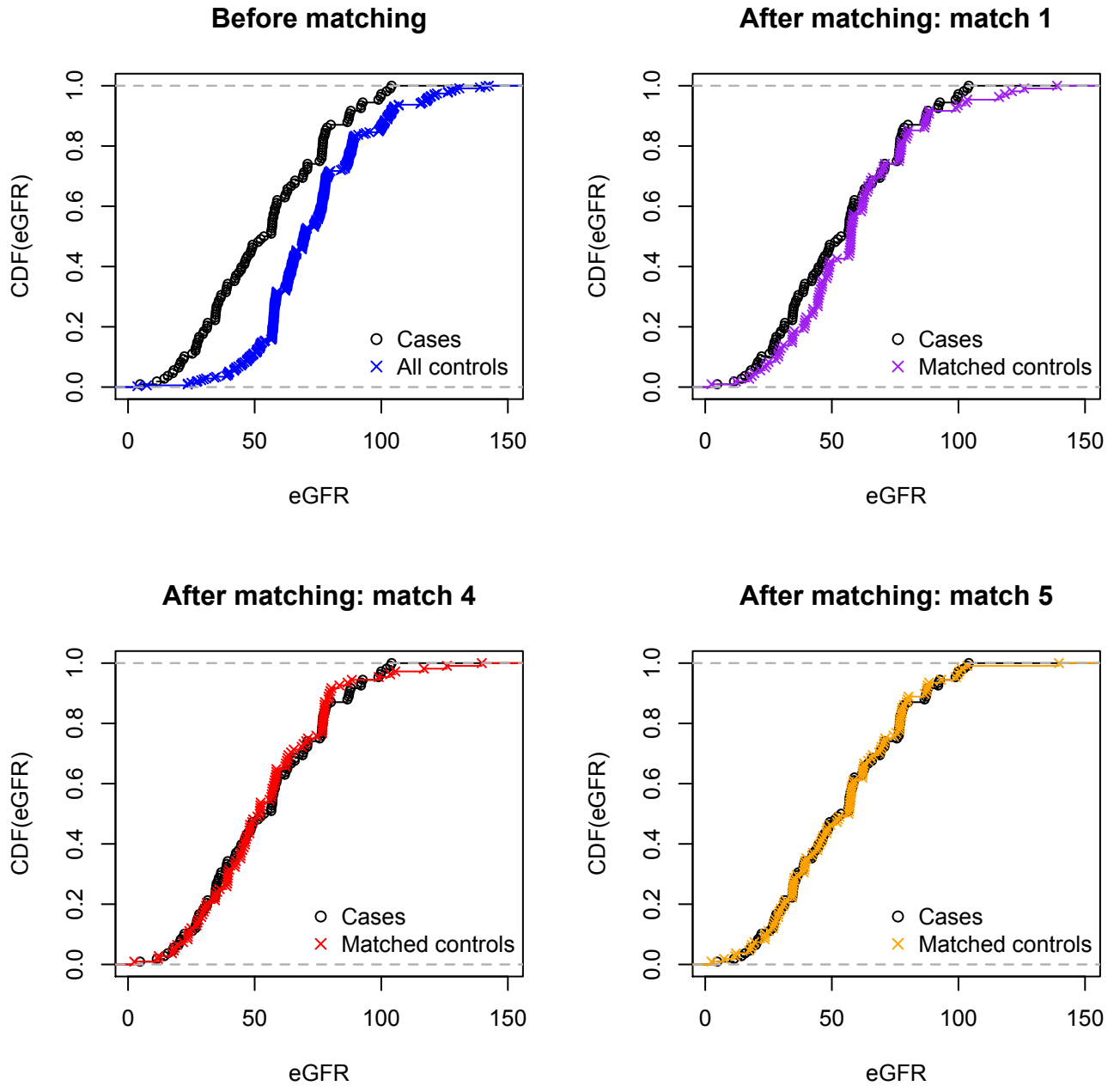
Figure 2: Balancing the K-S statistic for eGFR. Match 1 uses the assignment algorithm. Match 4 uses MIP to directly balance the means of all the covariates through the constraints with tolerances. Match 5 extends match 4 to balance both the means of all the covariates and the K-S statistic for eGFR using the constraint approach.
