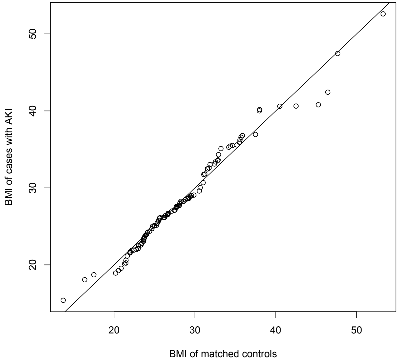
Figure 3: qq-plot of BMI for cases and matched controls.
