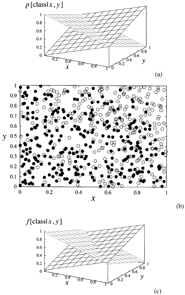
Figure 2. Example use of model trees for classification: (a) class probabilities for data generation; (b) the training dataset; (c) inferred class probabilities.
