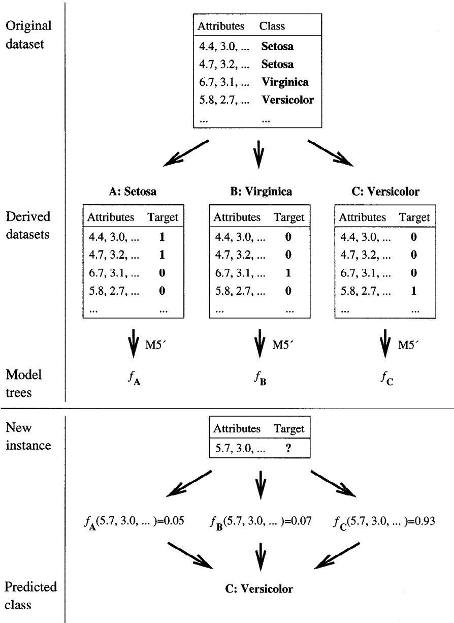
Figure 1. How M5' is used for classification.
