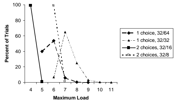
Fig. 2. One vs. two hash functions, over 10,000 trials. In the legend, the the number of items (in thousands) is followed by the number of buckets (in thousands).
