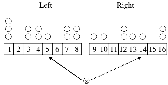
Fig. 1. The 2-left scheme. A newly inserted item, labeled z , is placed in the less filled of two random buckets, one from the left and one from the right. Ties are broken to the left. A search for z may require searching both of the buckets in which z might have been placed.
