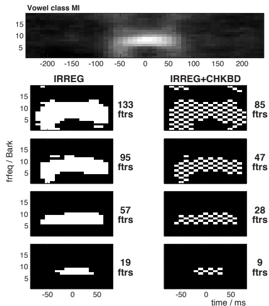
Figure 2: Mutual Information thresholded masks (IRREG) for features lengths 133,95,57,19 without checkerboarding (left) and features lengths 85,47,28,9 with checkerboarding (CHKBD, right).
