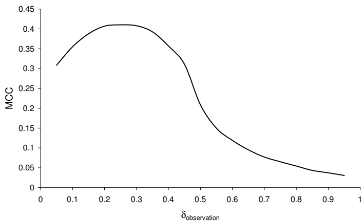
Figure 6.3: MCC with respect to the observation threshold ( \delta_{\text{observation}} )
