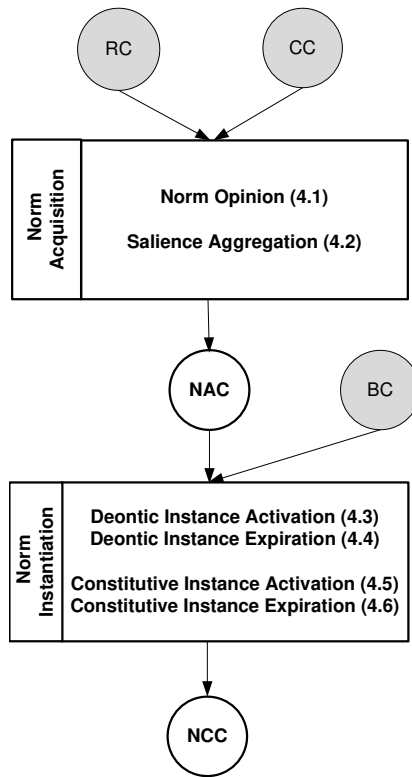
Figure 4.3: Representation of Norms and Instances in the n-BDI Architecture. In this image boxes have been split to show the names of the bridge rules that perform each task.
