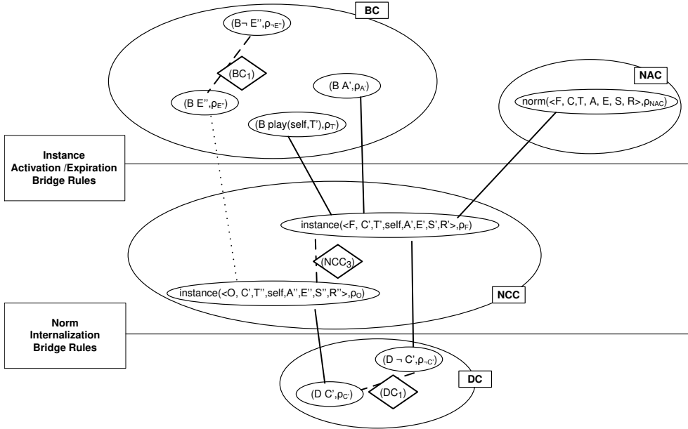
Figure 7.1: Coherence for normative reasoning. This image illustrates the BC, NAC, NCC and DC contexts. The coherence relationships among formulas that belong to a same context are defined by the inference rules of each context. Moreover, incoherence relationships among formulas belonging to a same context (broken lines) are defined by constraints, which are represented as rhombus, that have been added to the BC, NCC and DC. Finally, the coherence and incoherence relationships among formulas belonging to different contexts (represented as bold and dotted lines, respectively) are defined by means of the bridge rules that define the activation and expiration of norms and those bridge rules related to norm internalization.
