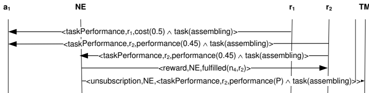
Figure 9.3: Observation of behaviours
