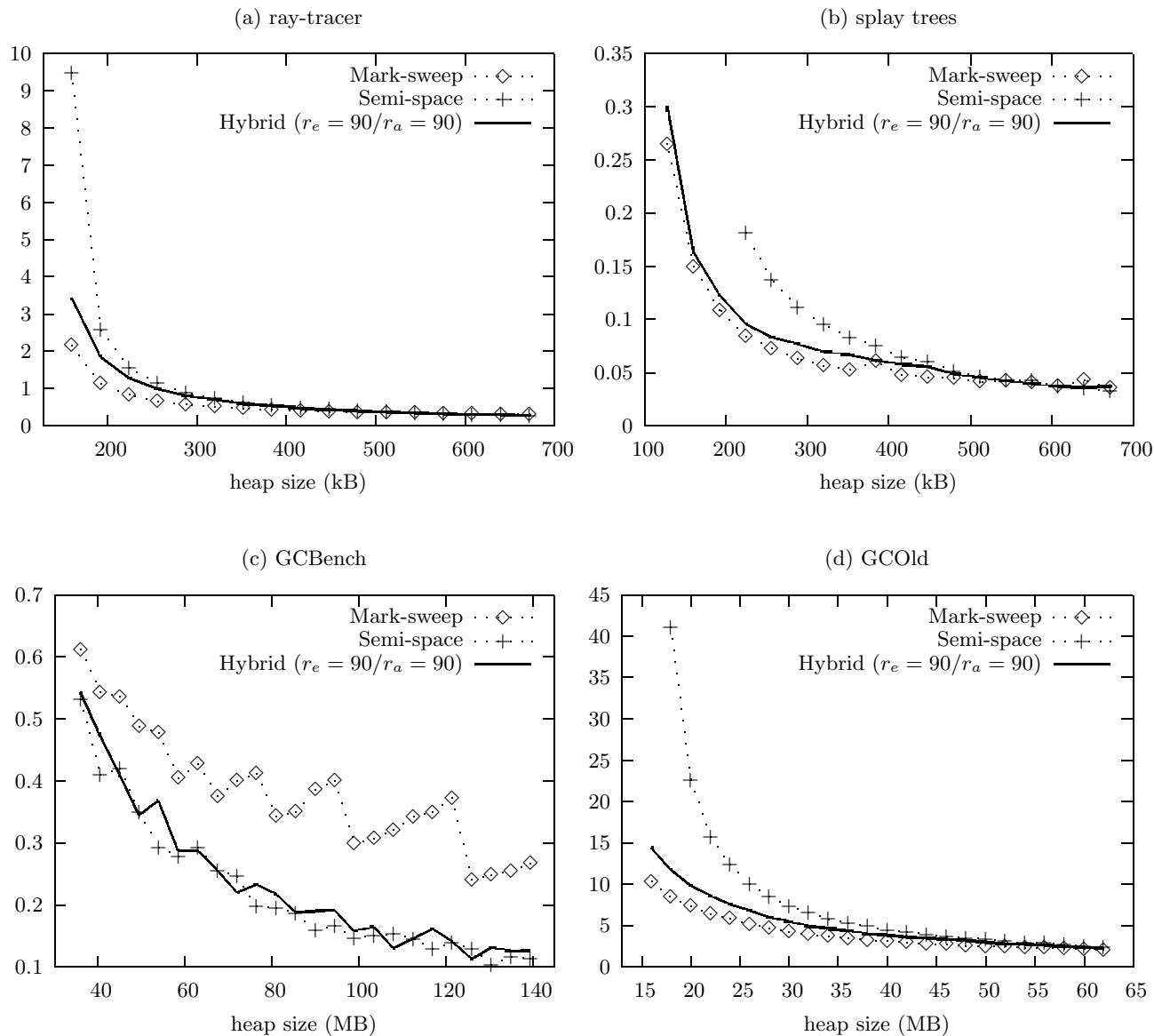
Figure 2: Collection Overhead vs. Heap Size. The vertical axis shows the total collection time measured in seconds. The same hybrid configuration is used in all cases ( r_e = 90\% and r_a = 90\% ). The jagged curve of mark-sweep collector in the GC Bench application is caused by the significant amount of garbage and strong correlation among object lifetimes in that application.
