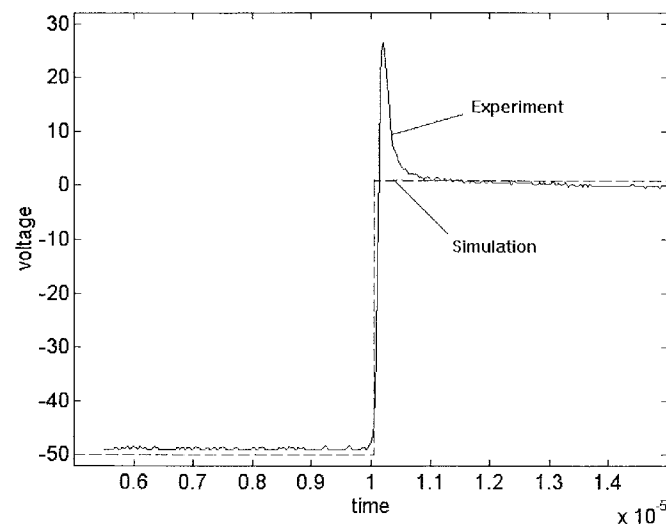
Fig. 2. Inability of SPICE diode model to simulate forward recovery in power diode voltage.
