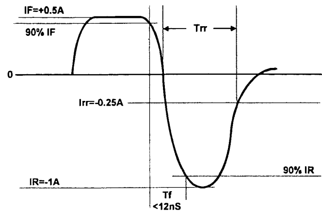
Fig. 3. Current waveform in RG1 reverse recovery test circuit.
