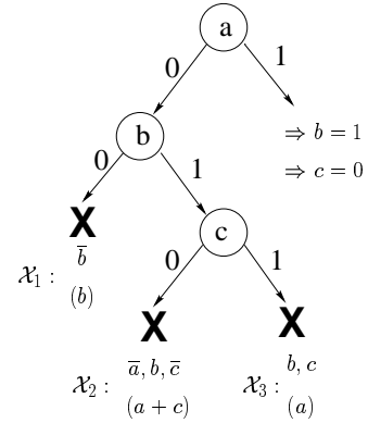
Figure 3. Symmetry in backtrack search
