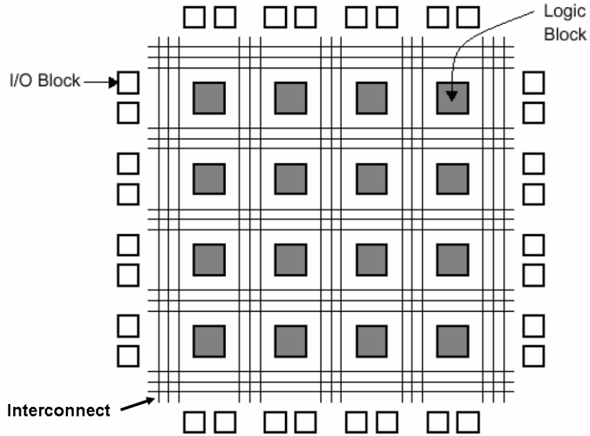
Figure 2.3: The Basic Structure of an FPGA [Kha02].
