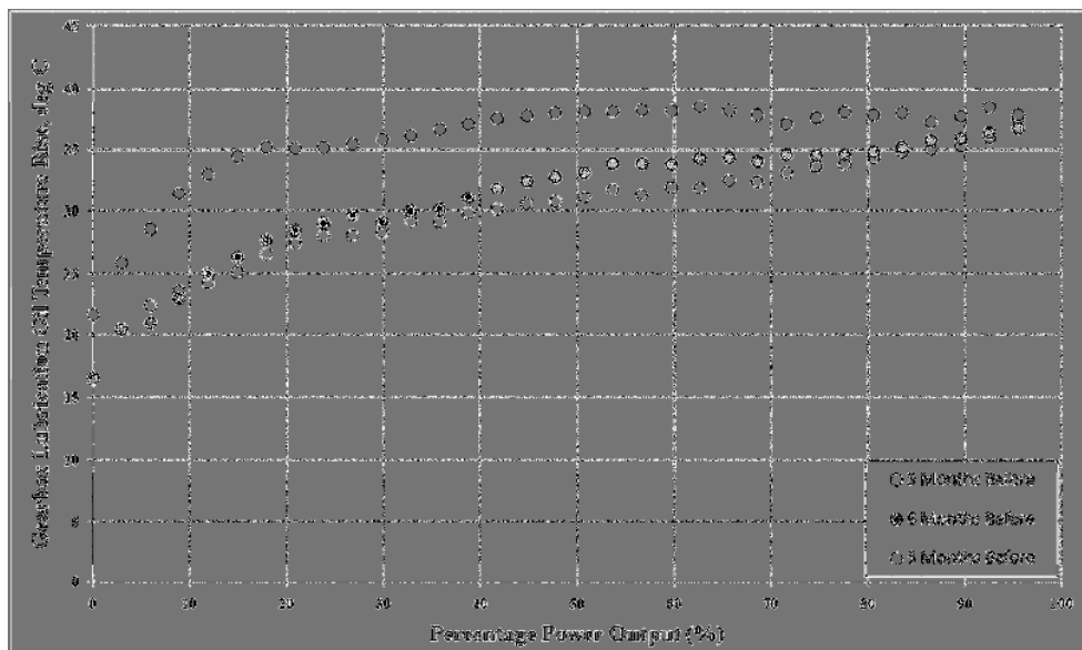
Fig. 1. Gearbox oil temperature rise by power bin during a developing failure from [24]. Reprinted from [24], Copyright 2012 with permission of John Wiley and Sons, Ltd.
