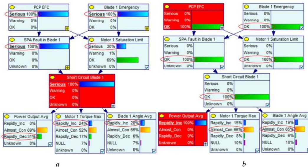
Fig. 11. Examples of Bayesian network reasoning from [62]. Reprinted with permission of [62]. Copyright 2012, Durham University.
