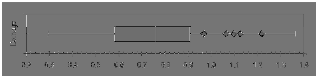
Fig. 7. Calculated bearing damage for 160 turbines from [55]. Box plot with extrema, quartiles and diamond symbols for failed turbines. Reprinted from [55], Copyright 2009 with permission of John Wiley and Sons, Ltd.
