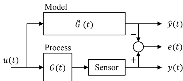
Fig. 4. Model-based monitoring with the input u(t) for both the process G(t) and its model \hat{G} , their outputs y(t) and \hat{y}(t) , respectively, and the final error or residual e(t) . Sketch adapted from [39].
