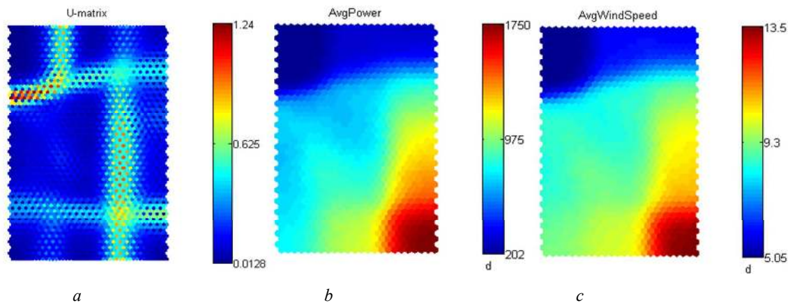
Fig. 3. General self-organizing map example from [28] showing in particular one cluster in the upper left and one in the lower right corner. Reprinted with permission of [28]. Copyright 2011, RES Offshore.
