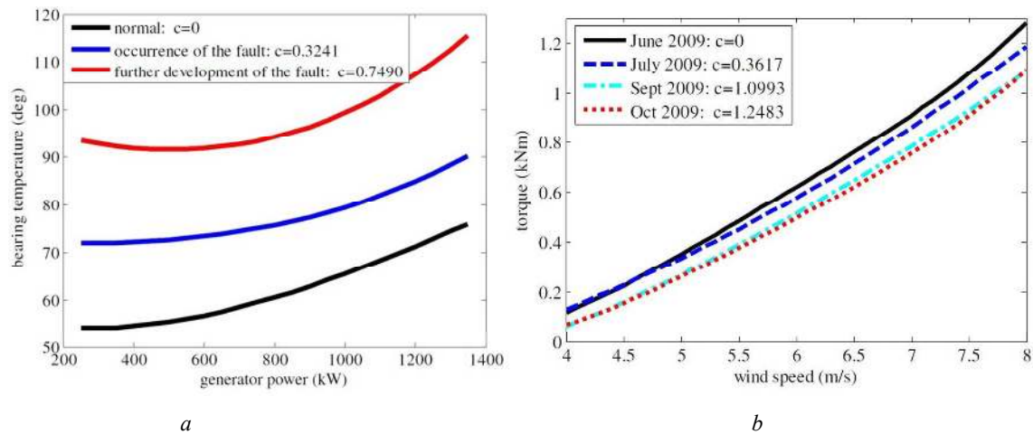
Fig. 2. Generator bearing fault detected through generator bearing temperature and blade deterioration detected through generator torque for different stages of the faults. Additionally, a calculated CM fault severity parameter 'c' is shown [4]. Reprinted from [4], Copyright (2013), with permission from Elsevier.
