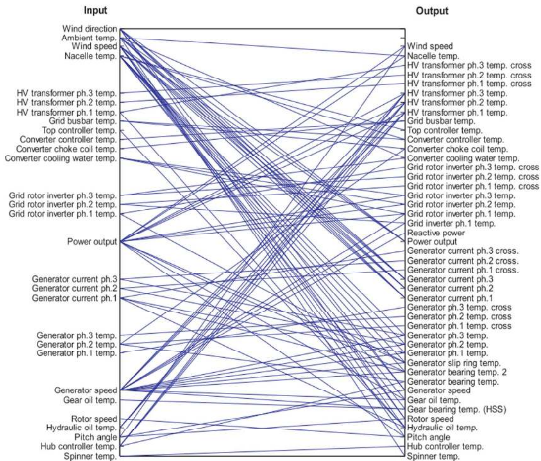
Fig. 6 Fuzzy modelling, input and outputs from [30]. Reprinted from [30], Copyright (2013) with permission from Elsevier.
