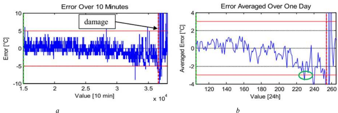
Fig. 5. Regression based generator bearing temperature modelling showing a catastrophic failure [40]. If the residual of measurement minus modelled temperature (“error”) is higher than the threshold, damage is likely. Reprinted from [40], Copyright (2010) with permission from Elsevier.
