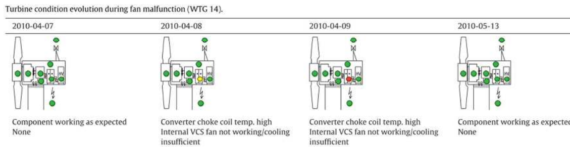
Fig. 12. Example of fuzzy expert system output from [51] giving component status as green (ok), yellow (warning) and red (alarm) and possible root cause. Reprinted from [51], Copyright (2014) with permission from Elsevier.
