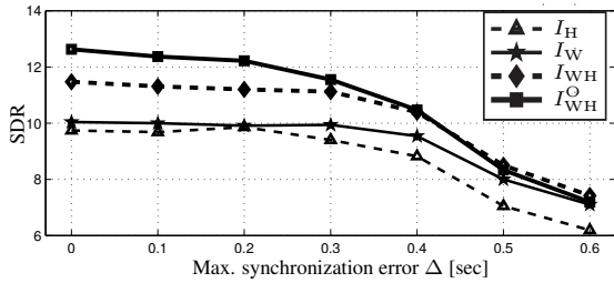
Fig. 4. Evaluation results given in SDR values for several separation approaches varying the synchronization error.
