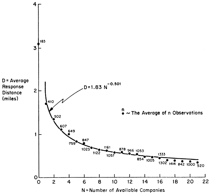
Figure 3. Simulated average response distances vs. the number of available companies (closest engine and ladder companies in the south Bronx).
