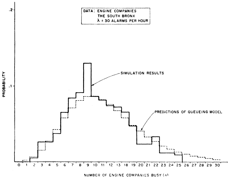
Figure 6. The probability that n engine companies are busy (south Bronx, \lambda = 30 ).
