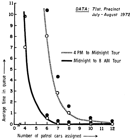
Figure 2. Delay in queue (in minutes) vs. number of patrol cars assigned; ● = simulation results, ○ = predictions of queuing model.
