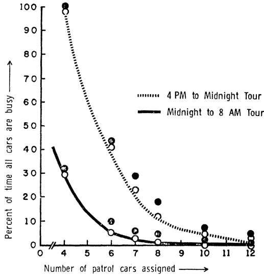
Figure 1. Unavailability of patrol cars vs. number of cars assigned; ● = simulation results, ○ = predictions of queuing model.
