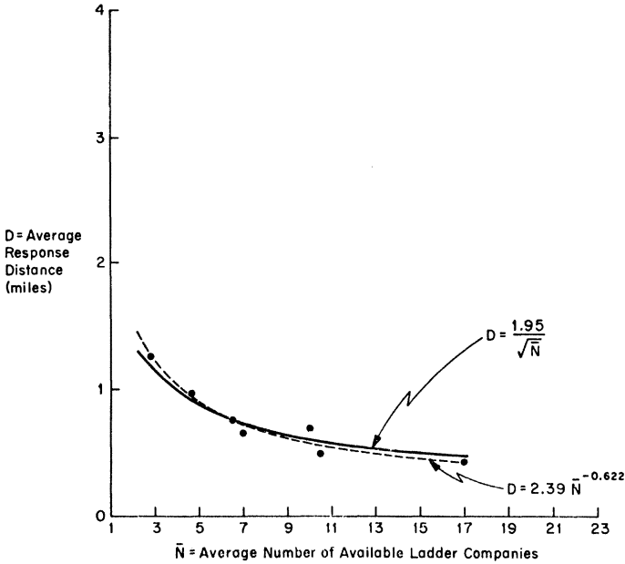
Figure 4. Simulated long-run average response distance vs. the average number of available companies (closest ladder companies in the south Bronx).
