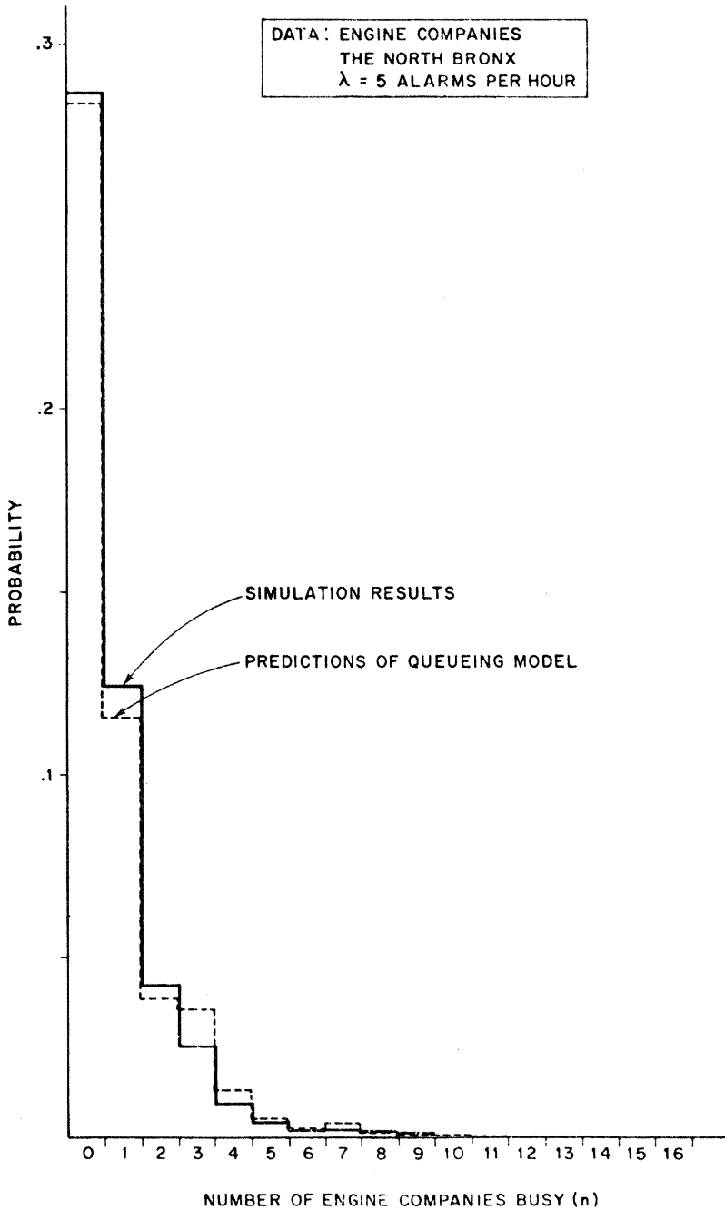
Figure 5. The probability that n engine companies are busy (north Bronx, \lambda = 5 ).
