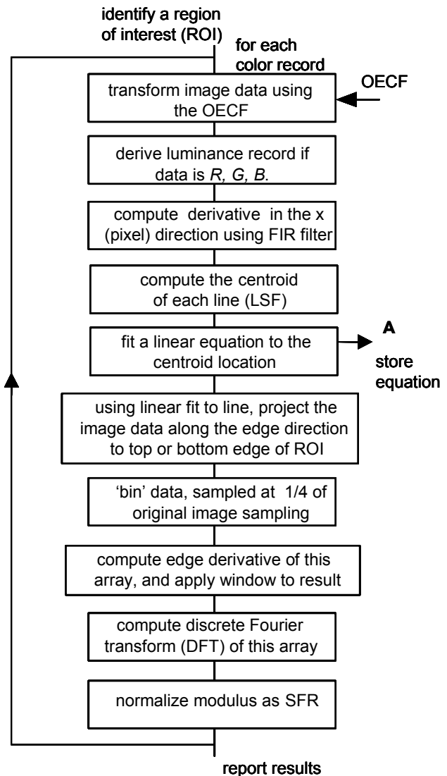
Figure 1: A description of the ISO 12233 Spatial Frequency Response evaluation. Storage of the equation for the edge at step A has been added. The edge is assumed to be oriented in a near-vertical direction. Figure has been edited to correct an error in the published PICS 1999 Proceedings.
