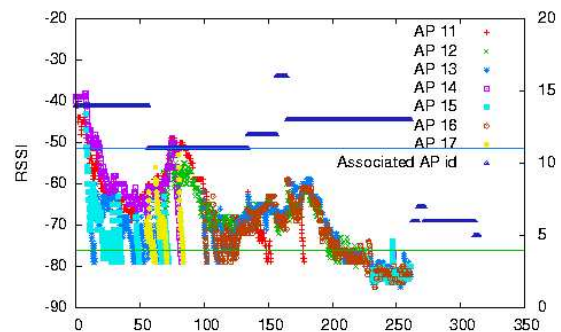
Figure 7: RSSIs as seen by the client when operating on channel 11, and corresponding handoffs with Hysteresis scheme.
