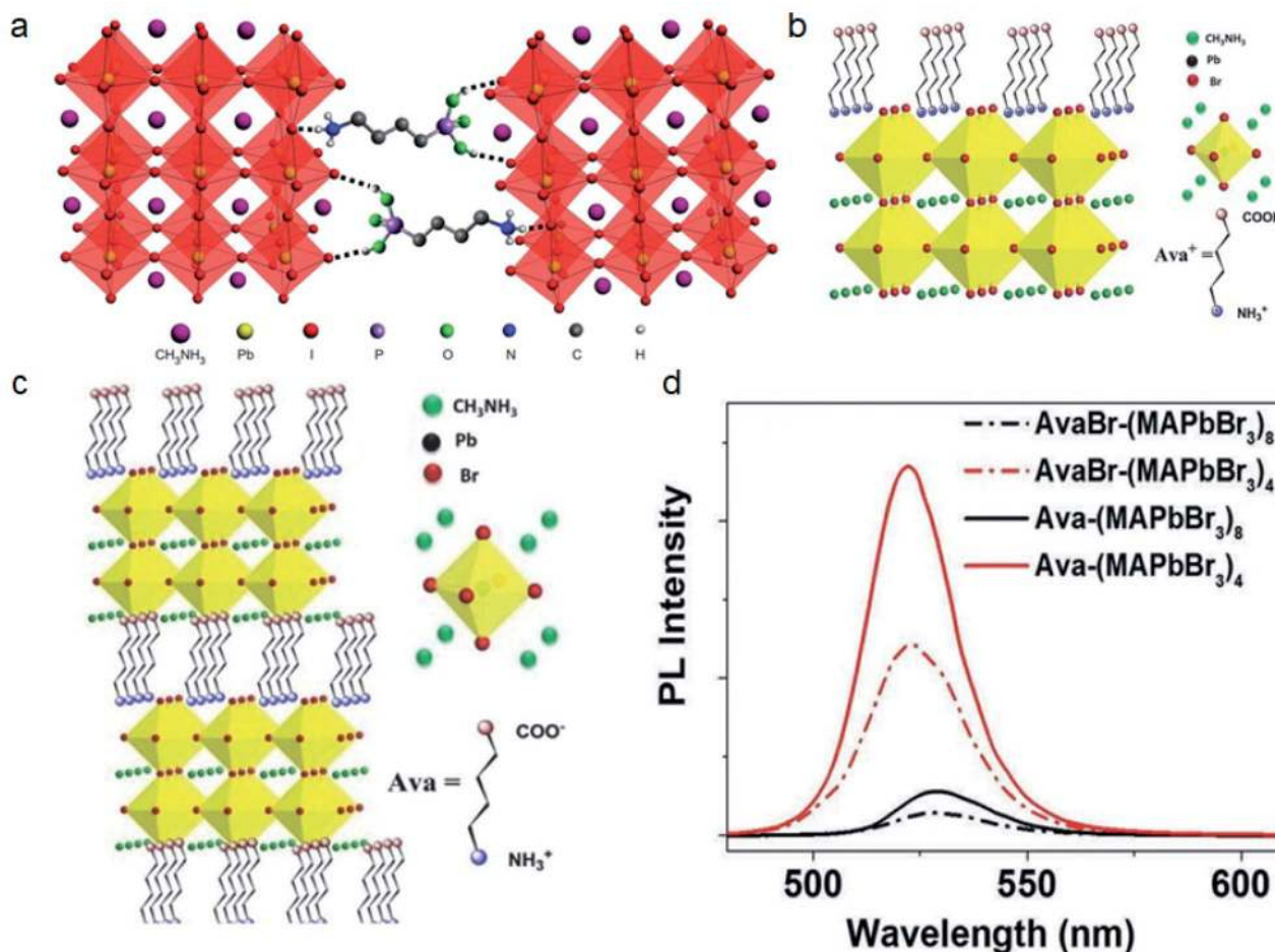
Fig. 10 (a) 3D perovskites cross-linked by 4-ABPAOI. Reproduced with permission from ref. 138. Copyright 2015 Springer Nature. (b) 5-Ava perovskites cross-linked by Pb–COO bonds and interactions between \text{NH}_3^+ and [\text{PbBr}_6]^{4-} units. (c) Single linked 5-AvaBr on 3D perovskites. (d) PL spectra of 5-Ava and 5-AvaBr treated perovskite films. Reproduced with permission from ref. 139. Copyright 2017 John Wiley and Sons.
