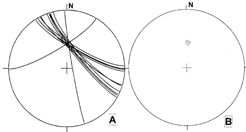
Figure 2. Small circles (A) and confidence regions at 95 per cent and 63 per cent (B) associated with the syntectonic remagnetization determined by Henry et al. (2001) and Rouvier et al. (2001) on the Cévennes border. Stereographic projection in the lower hemisphere.
