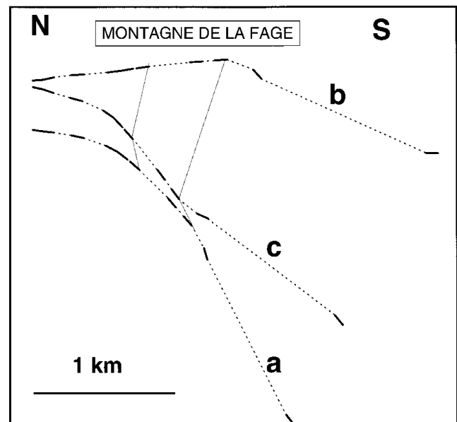
Figure 7. Cross-section presenting folding of the same bed in the Montagne de la Fage fold: (a) present state (see text) and (b) during remagnetization. (c) Deformation, undergone after the remagnetization, of a plane which would have been horizontal during the remagnetization.
