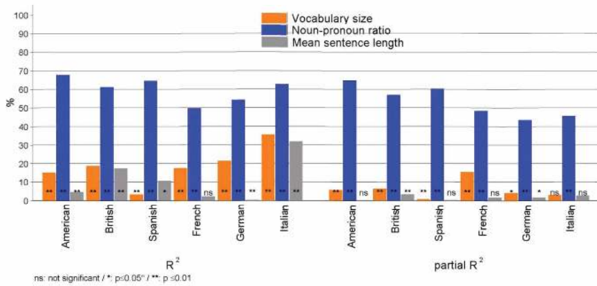
Figure 13: Coefficients of determination (left side) and partial coefficients of determination (right side) between year-to-year changes of a_{ZM} and year-to-year changes of the vocabulary size (orange), the noun–pronoun ratio (blue) and the mean sentence length (gray) for all six investigated languages. Word types with a frequency of less than ten were excluded from this analysis.
