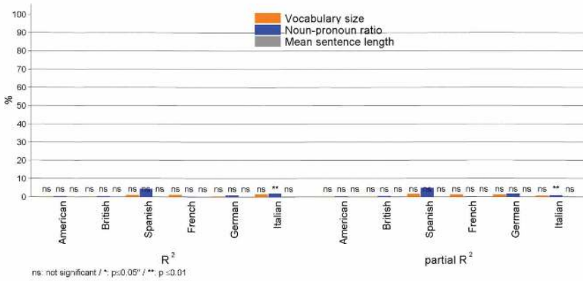
Figure 11: Coefficients of determination (left side) and partial coefficients of determination (right side) between year-to-year changes of power law (using the method presented in Clauset et al. (2007)) exponent and year-to-year changes of the vocabulary size (orange), the noun–pronoun ratio (blue) and the mean sentence length (gray) for all six investigated languages.
