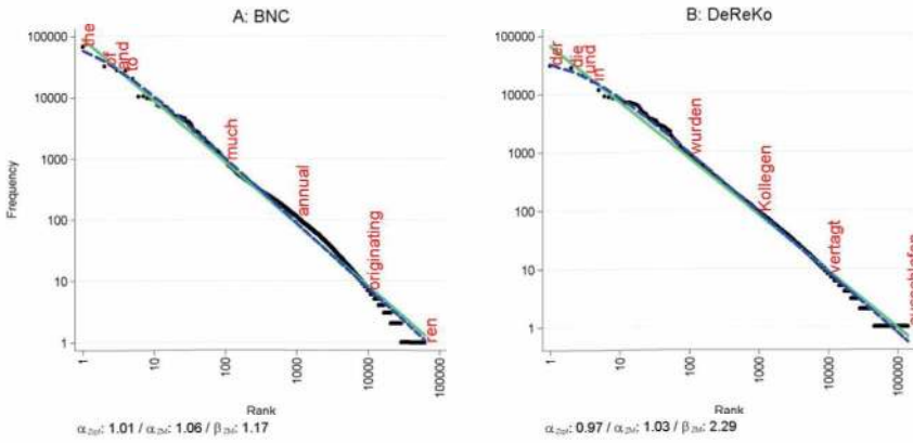
Figure 1: Two word frequency distributions (1 million samples in each case). Plot A: data from the British National Corpus. Plot B: data from the German Reference Corpus. The black dots represent the empirical data; the solid mint line represents the fit to a Zipf distribution; the blue dashed line represents the fit to a Zipf–Mandelbrot distribution. The fitting and sampling procedure is described in the text. The parameters of the distributions are added as a note. Some examples are depicted in red.
