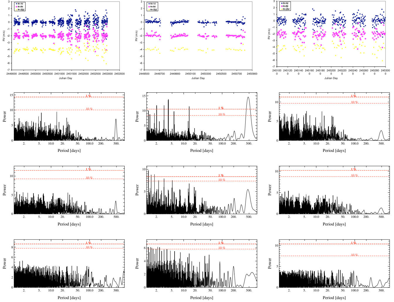
Fig. 15. Impact of the data sampling: Top : RV of a spotted solar-type star surrounded by a 1 M_{\text{Earth}} planet orbiting at 1.2 AU. The star is assumed to be observable 8 months per year and observed every 4 days ( top data ); 8 days ( middle data ) or 20 days ( lower data ). In all cases, we assume a precision of 5 cm/s. The RV curves have been vertically shifted for clarity purposes). The full cycle ( left ) as well as a low activity ( middle ) and high activity ( right ) periods are considered. The corresponding periodograms are provided: first line: temporal sampling is 4 days; second line: 8 days and third line 20 days.
