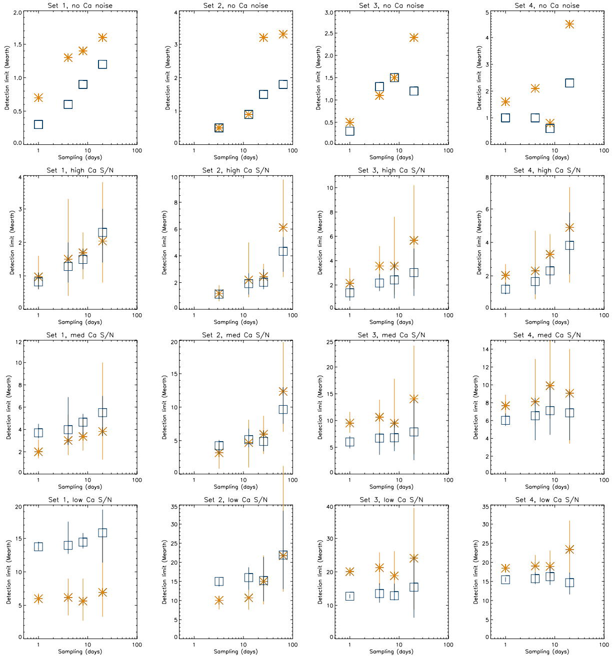
Fig. 15. Detection limits versus sampling for the corrected signal using reconstructed Ca for the correlation-based method (stars, orange), and the LPA method (squares, blue). Each row corresponds to a different Ca noise level (from top to bottom: no noise, \sigma_{\text{high}} , \sigma_{\text{med}} , \sigma_{\text{low}} ). Each column corresponds to a data set (from left to right: from Set 1 to Set 4). The errorbar symbols indicate the minimum value and maximum values for each detection limit, computed for ten realisations of the Ca noise.
