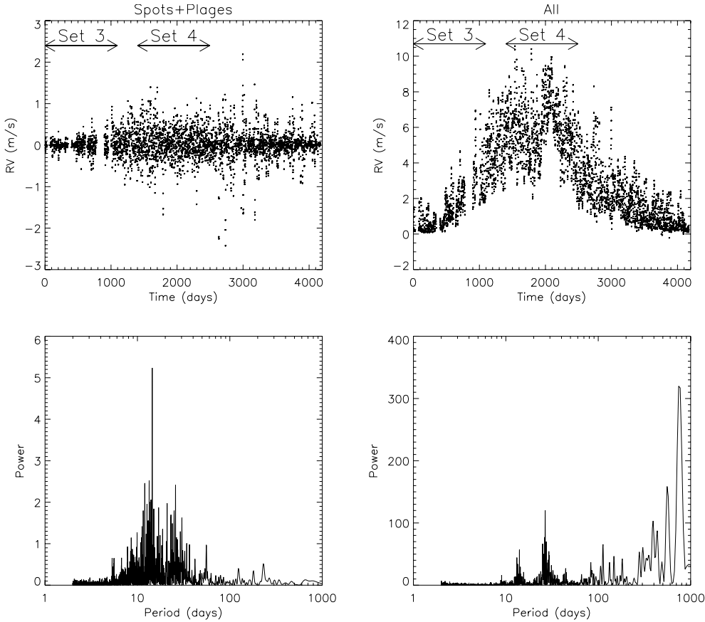
Fig. 1. Upper panels: reconstructed series for spots+plages RV_{\text{sppl}} (left) and all components including convection RV_{\text{tot}} (right). Set 3 and Set 4 are indicated by horizontal arrows. Set 1 and Set 2 cover the whole range. Lower panels: corresponding periodograms. The periodograms are in the same arbitrary units.
