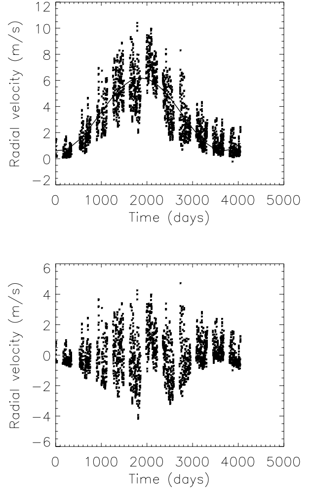
Fig. 10. Upper panel: RV_{\text{tot}} versus time for Set 1, best sampling. The solid line is the sinusoidal fit derived as described in Sect. 4.1. Lower panel: RV after correction using the sinusoidal fit method, assuming no Ca noise.
