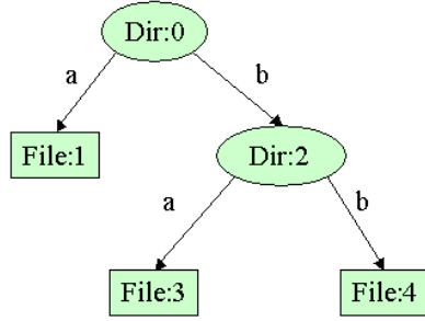
(a) Initial tree
