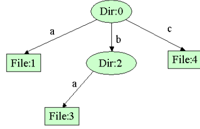
(b) tree after mv(2, 4, b, 0, c)
