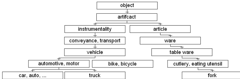
Figure 1. Hyponym taxonomy in WordNet used for path length similarity measurement [5,6]:
