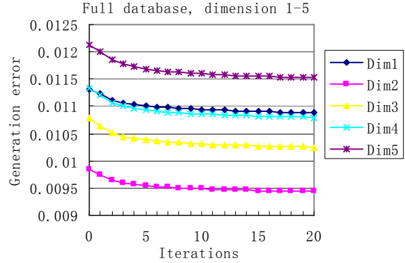
Figure 3: Convergence of MGE training
