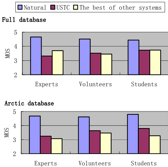
Figure 4: Average MOSs of natural speech, USTC system and the best of other systems
