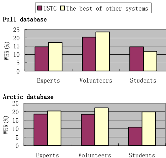
Figure 5: Average WERs of USTC system and the best of other systems
