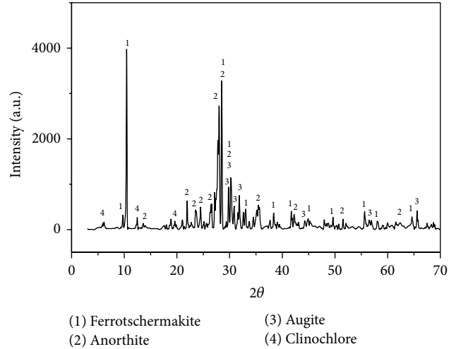
FIGURE 1: The XRD pattern of IOT.
