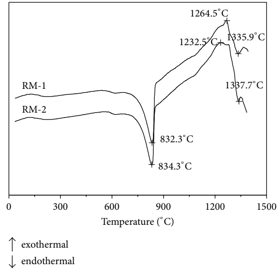
FIGURE 2: The DSC heating curves of raw meals.
