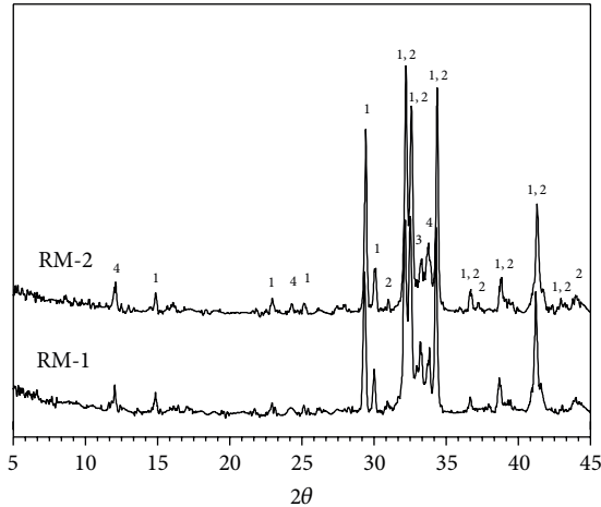
(1) \text{C}_3\text{S} -Alite (2) \text{C}_2\text{S} -Belite (3) \text{C}_3\text{A} -Aluminate (4) \text{C}_4\text{AF} -Ferrite
