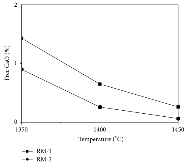
FIGURE 3: The burnability tests of raw meals.
