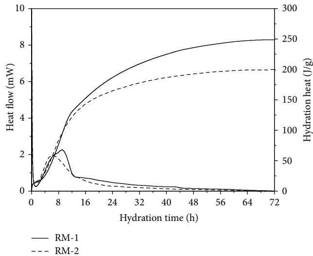
FIGURE 6: The hydration heat of two produced Portland cement clinkers.
