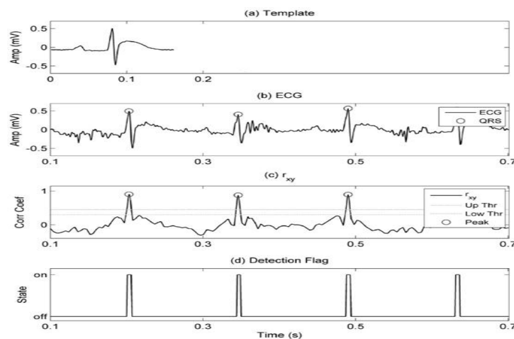
Figure 2. Template matching for QRS detection
