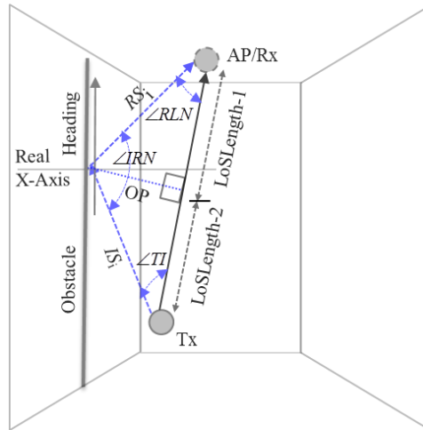
Figure 7. An Example of a Reference Length of LoS Estimation in Case of \angle IRN is 90^\circ < (\angle IRN) < 180^\circ in Wireless Indoor Scenario
