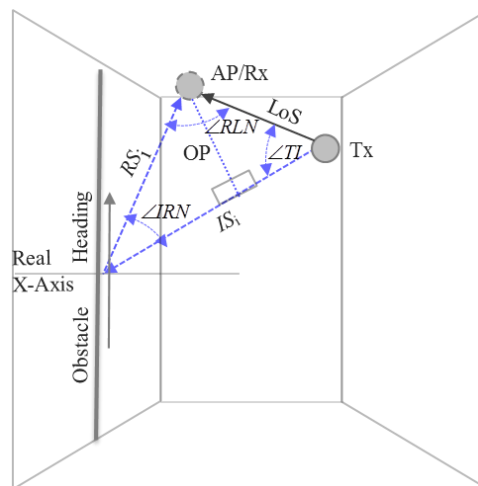
Figure 8. An Example of a Reference Length of LoS Estimation in Case of \angle IRN is 0^\circ < (\angle IRN) < 90^\circ in Wireless Indoor Scenario
