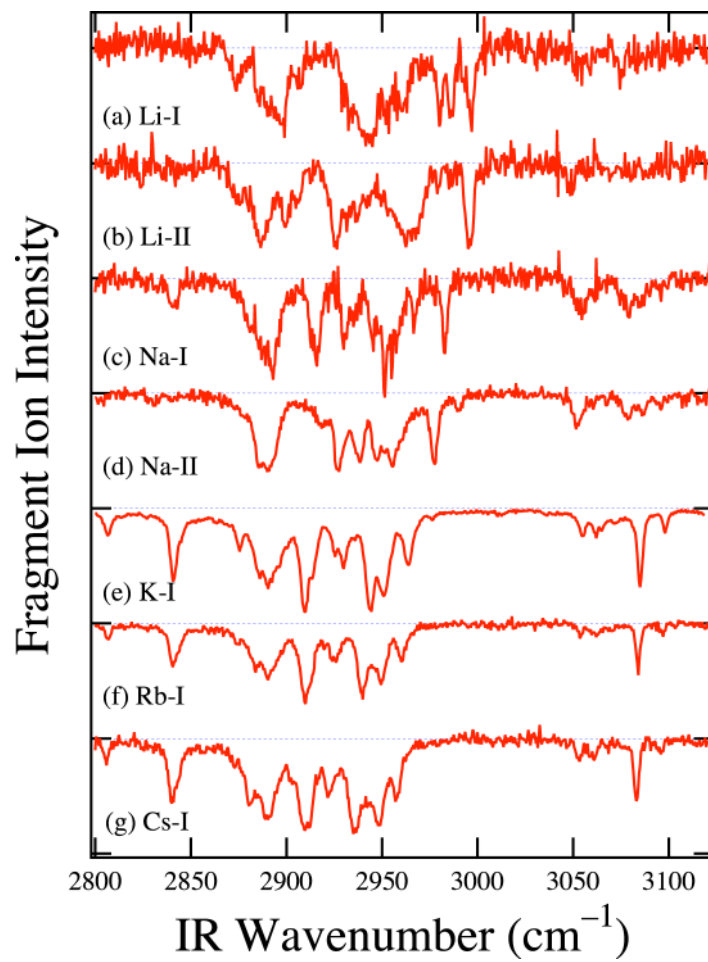
Figure 4. The IR-UV double-resonance spectra of the M^+\bullet\text{DB18C6} ( M = \text{Li}, \text{Na}, \text{K}, \text{Rb}, \text{and Cs} ) complexes in the CH stretching region.
