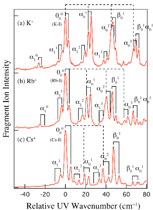
Figure 3. The UVPD spectra of the DB18C6 complexes with K^+ , Rb^+ , and Cs^+ around their respective origin bands. The horizontal axis is the UV wavenumber relative to the band origin. The doublet structure connected by solid lines is attributed to the exciton splitting due to the intramolecular interaction between the benzene rings. The low-frequency vibrations appearing in these spectra are labeled by \alpha and \beta . Superscript and subscript integers with \alpha and \beta denote quantum numbers of these vibrations in the S_1 and S_0 states, respectively. Progressions of vibrations \alpha from the origin band are presented with dotted lines.
