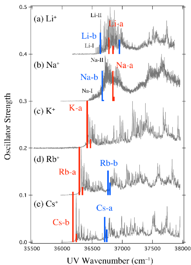
Figure 7. Oscillator strengths of electronic transitions for M^+\bullet\text{DB18C6} ( M = \text{Li, Na, K, Rb, Cs} ) calculated with TD-DFT at the M05-2X/6-31+G(d) level and the Stuttgart RLC potential for Rb and Cs. Calculated transition energies are scaled with a scaling factor of 0.8340 in order to compare the calculated and experimental spectra. The scaling factor is determined so as to reproduce the transition energy of the origin band of \text{K}^+\bullet\text{DB18C6} .
