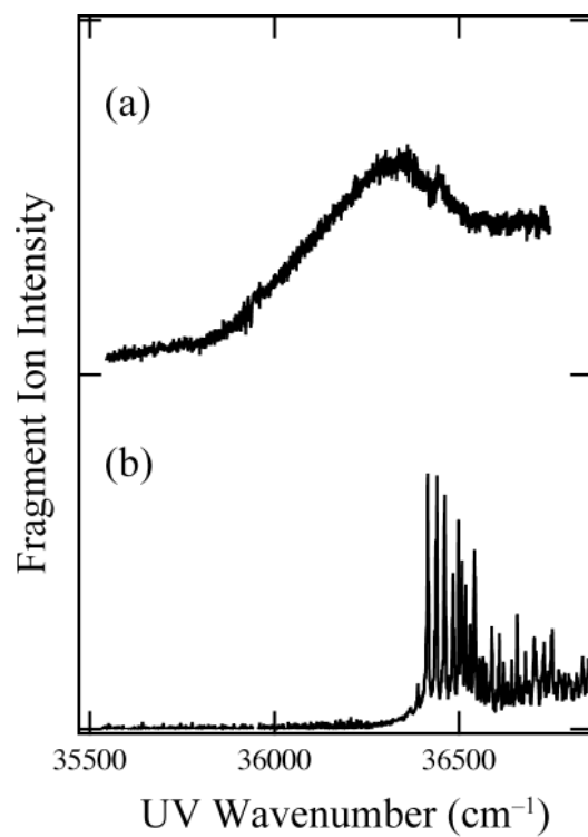
Figure 1. The UVPD spectra of (a) uncooled \text{K}^+\cdot\text{DB18C6} and (b) \text{K}^+\cdot\text{DB18C6} that is cooled in the 22-pole ion trap. The temperature of the cooled complex is estimated to be \sim 10 K.
