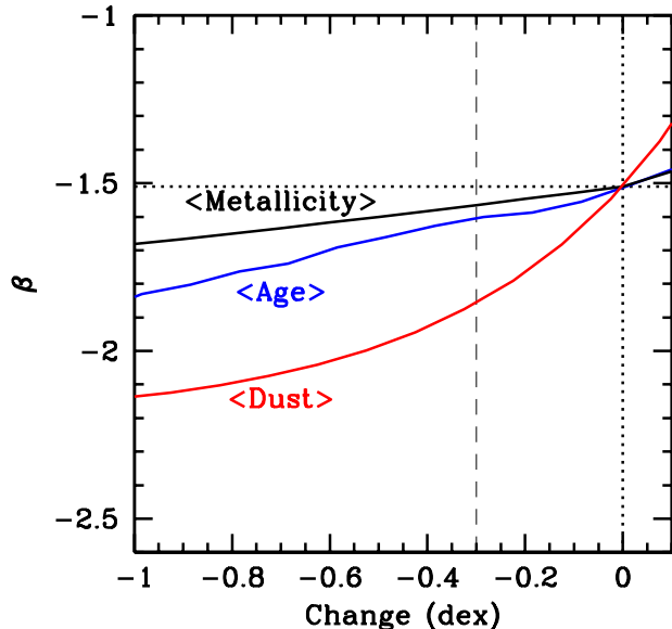
FIG. 7.— UV -continuum slope \beta ( 1600\text{\AA} to 2300\text{\AA} rest-frame baseline) predicted for specific fractional changes in the mean age, metallicity, or dust extinction of high-redshift star-forming galaxies from our fiducial stellar population model. For our fiducial model (where \beta = -1.47 ), we assume t = 70 Myr, \tau = 10 Myr, [Z/Z_{\odot}] = -0.7 , E(B - V) = 0.15 , and a Salpeter IMF (where the star formation history is parametrized as e^{-t/\tau} ) from the Papovich et al. (2001) fits to z \sim 2.5 U -dropouts from the WFPC2 HDF North. In modifying our fiducial model to have younger ages, we make changes to both t and \tau . A factor of 2 (0.3 dex) change (dashed line) in the mean dust content, age, or metallicity of the star-forming galaxy population at high redshift shifts the UV -continuum slope \beta by \sim 0.35 , \sim 0.1 , and \sim 0.05 , respectively. The effect of the stellar IMF on \beta is not shown here, but results in only modest changes in \beta , i.e., \Delta\beta \lesssim 0.1 for a \sim 0.5 shift in the slope of the IMF. It seems clear that changes in the mean dust content of galaxies at high-redshift has the biggest effect on the UV -continuum slope \beta – though some change is also likely the result of differences in the average age. Nonetheless, since stellar population modelling of z \sim 4 - 6 dropout galaxies (Stark et al. 2009) suggest that age shows little dependence on redshift or luminosity (at least in the median), it seems likely that age only plays a minor role ( \Delta\beta \lesssim 0.2 ) in driving the observed trends (§4.4).
