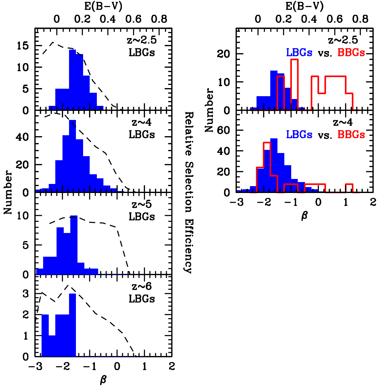
FIG. 6.— ( left ) Distribution of UV -continuum slopes \beta observed at z \sim 2-6 for the present Lyman-Break Galaxy selections (solid blue histograms). We only include the observed \beta values for Lyman-Break galaxies >1 mag brighter than the selection limit to avoid being dominated by selection effects. On the top axes are the E(B-V) extinctions (Calzetti et al. 2000 law) that are equivalent to a given \beta if the base spectrum is a young star-forming galaxy ( \sim 100 Myr of constant star formation). The selection volume (§3.7) available for galaxies with UV -continuum slope \beta and magnitudes \gtrsim 1 mag brighter than the selection limit is shown with the thick dashed lines in each panel (the normalization is arbitrary). While it is more difficult to select galaxies with redder UV -continuum slopes \beta with a Lyman Break criterion, our simulations (§3.7) indicate that our dropout selections should be capable of identifying modest numbers of galaxies with \beta 's as red as 0.5. Indeed, such galaxies (with \beta 's redder than -1 ) are present in our z \sim 2-4 LBG selections albeit in small numbers. However, they are conspicuously absent in our z \gtrsim 5 selections. This suggests that such sources are exceedingly rare at z \gtrsim 5 . Conversely, the modest number of galaxies with red UV -continuum slopes \beta 's seen at z \sim 4 seem consistent with the small samples of z \sim 4 ULIRGs that have been found in the observations (e.g., Daddi et al. 2009). The lack of very blue \beta \lesssim -3 galaxies is also consistent with expectations from models and suggest that the \beta distributions derived here are reliable. ( right ) Distribution of UV -continuum slopes observed for Lyman Break Galaxy selections at z \sim 2-4 (solid blue histogram) and for Balmer-Break Galaxy selections at z \sim 2-4 (red histogram: Brammer & van Dokkum 2007). The E(B-V) extinctions given on the top axis are as in the left panel (but are not expected to be particularly representative for the somewhat older BBGs). Both \beta distributions plotted are as observed, with no correction for selection or measurement effects. Balmer-Break Galaxy (BBG) selections provide us with an independent measure of the UV -continuum slope distribution since they do not depend upon their UV -continuum slope or the brightness of these sources in the UV -continuum. The fact that the distribution of UV -continuum slopes \beta is becoming substantially bluer for both selections (and in particular the Brammer & van Dokkum 2007 BBG selection at z \sim 4 ) suggests that Lyman-Break selections (sensitive to galaxies with \beta 's bluer than 0.5: see Figures 2 and 4) should be largely complete at z \gtrsim 5 (see §4.2).
