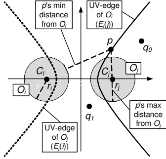
Fig. 3. The UV-edge.
