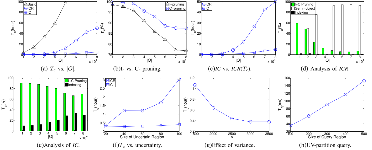
Fig. 7. UV-Diagram Analysis
