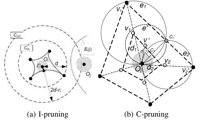
Fig. 4. Our pruning methods.
