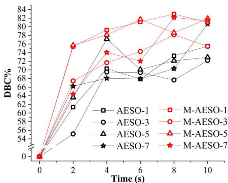
Figure 3. Double bond conversion (DBC%) rate as function of the UV-curing time for neat AESO and M-AESO for different loading of the photoinitiator.
