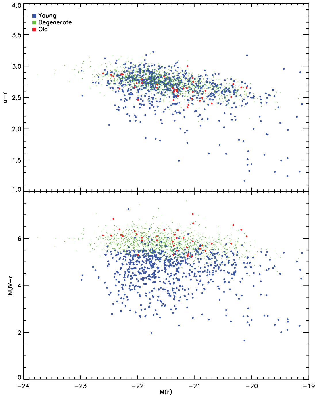
FIG. 11.—Optical u - r CMR ( top panel ) and the NUV CMR ( bottom panel ) for the GALEX early types color-coded using the following classification scheme: if the 95% confidence contour does not extend to ages higher than 1 Gyr then the galaxy is classified as young (e.g., galaxies 1 and 2 in Fig. 8); if the 95% confidence contour spans ages below and above 1 Gyr, the galaxy is classified as degenerate (e.g., galaxy 3 in Fig. 8); if 95% confidence contour lies exclusively above an age of 1 Gyr, then the galaxy is classified as old (e.g., galaxy 4 in Fig. 8). Young galaxies are shown in blue, intermediate galaxies are shown in green and old galaxies are shown in red. Note that the photometry has not been K -corrected because this requires the assumption of a template—it is evident that an old passively evolving population is not good template for the local early-type population, at least for UV photometry.
