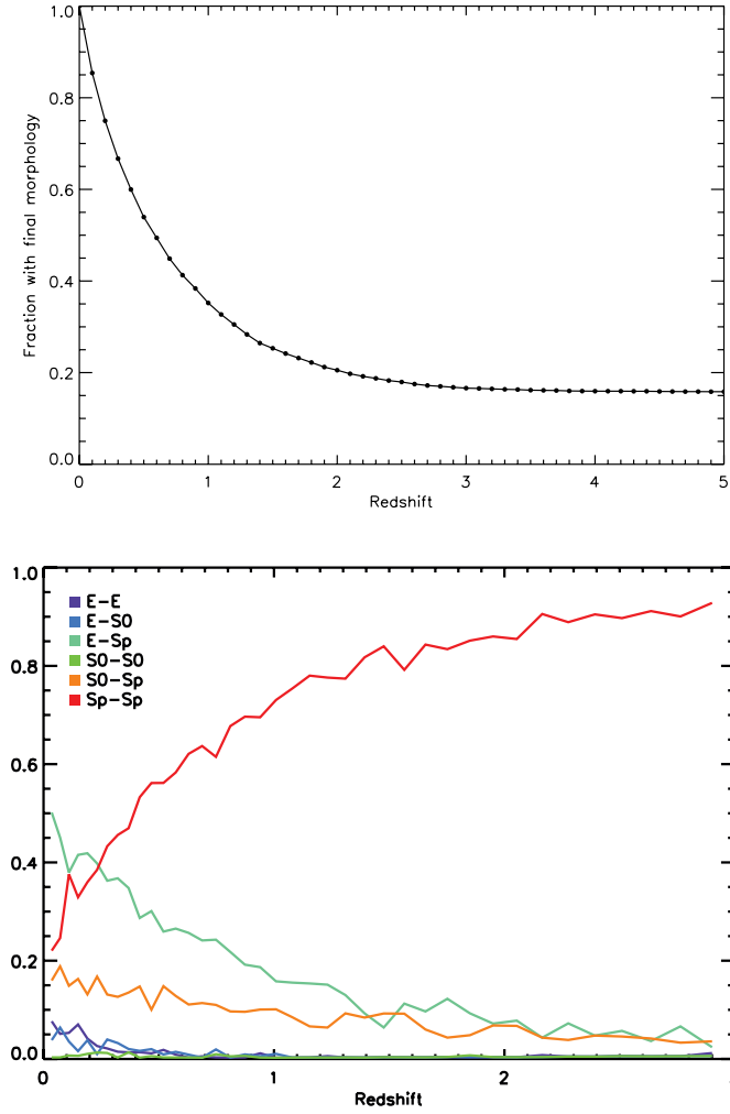
FIG. 25.— Top : Fraction of local ( z = 0 ) early-type galaxies that have already attained their final (early-type) morphology, i.e., had their last merger, as a function of redshift. Bottom : Progenitor types in binary mergers. At low redshift mergers have a higher probability of having at least one early-type progenitor. See Khochfar & Burkert (2003) for a detailed analysis of the progenitor morphologies of early-type galaxies.
