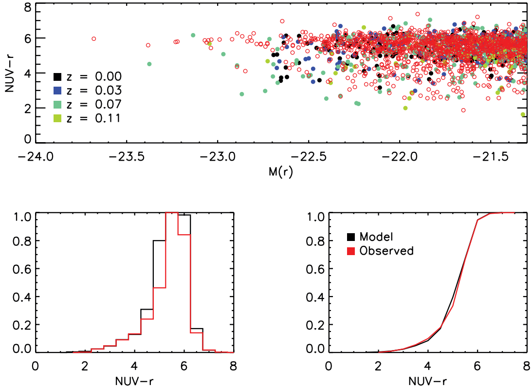
FIG. 19.—Comparison of observed and model photometry in the best-fit model where \mu = 3 , \tau_{\max} = 30 Myr (see Charlot & Fall 2000) l_{\min} = 20 Myr and l_{\max} = 200 Myr. The open red circles represent the observed photometry. All other colors represent model galaxies at various redshifts (see legend in plot). The bottom panels condense the information shown in the top panel. The plot on the bottom left shows the NUV - r color distribution and the plot on the bottom right shows the cumulative NUV - r color distribution.
