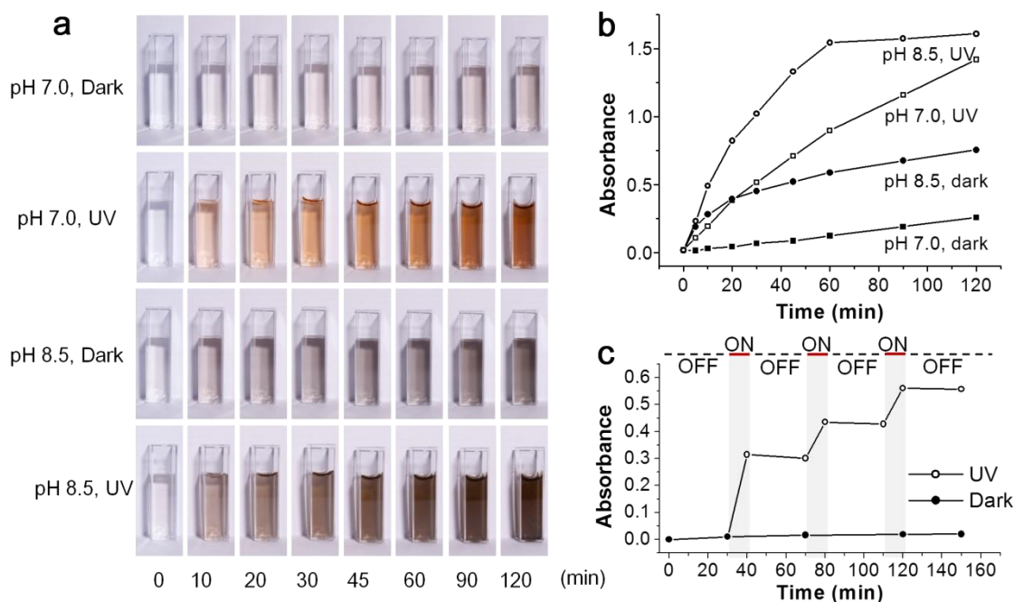
Figure 2 Color and absorbance change of dopamine solutions. a) Photographs of the corresponding dopamine solutions at different time points. b) Absorbance of the dopamine solution (2 mg/ml) at 420 nm as a function of time and pH. c) Change of absorbance (at 420 nm) of a low oxygen containing dopamine solution under UV irradiation at 254 nm (○) and in the dark (●). Dopamine solution (pH 7.0, purged with argon for 10 min) was irradiated for 10 min, followed by 30 min in the dark. The cycle was repeated 3 times.
