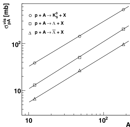
Fig. 4 Atomic mass number dependences of the V^0 integrated inclusive cross sections \sigma_{pA}^{\text{vis}} . The solid lines represent fits to the parameterization (Eq. 4). The uncertainties include both statistical and systematic contributions
