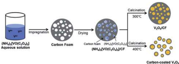
Fig. 12 Schematic of the preparation of carbon-fabricated V 2 O 5 samples (CF300 and CF400). 117
