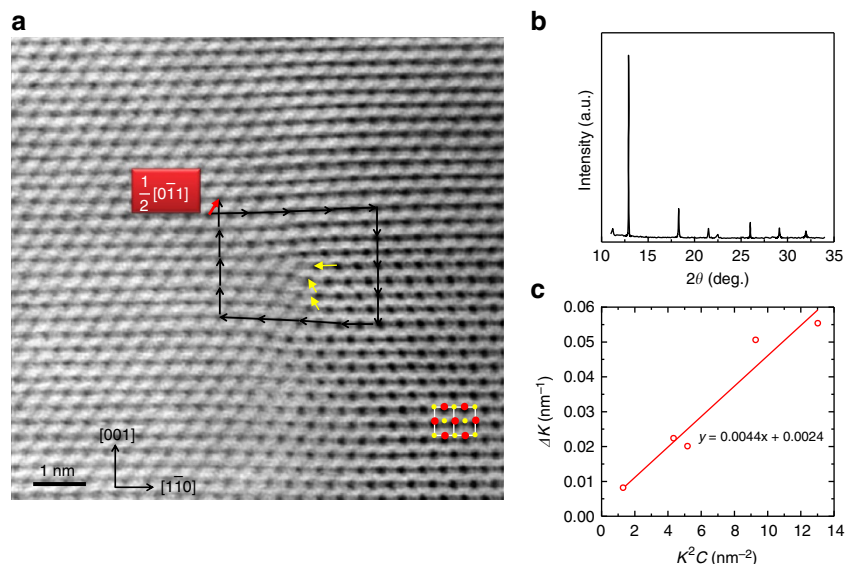
Figure 2 | The feature of the dislocation and synchrotron diffraction results for Pb_{0.95}Sb_{0.033}Se solid solution. A high-resolution annular bright field (ABF) STEM image (a) shows the detailed dislocations in the sample with x = 0.05 . The black arrows give a complete Burgers loop of a dislocation and the yellow arrows show one (001) and two (111) extra half planes of atoms. The estimated Burger's vector (red arrow) for the observed dislocations is B_D = 1/2[0\bar{1}1] . The inset shows the structural model of PbSe projected in [1\bar{1}0] direction with red dots standing for Pb , whereas yellow ones for Se . Neither precipitates nor nanometre-scale grains are observed. The synchrotron XRD pattern (b) and the peak broadening analysis by the modified Williamson-Hall plot (red line) in which the slope and intercept reveal the dislocation density and the crystallite size (c).
