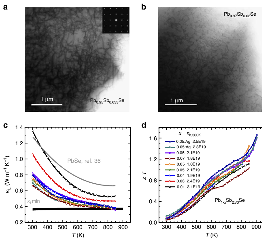
Figure 1 | Microstructures and thermoelectric properties. Uniformly distributed dense dislocations in Pb_{0.95}Sb_{0.033}Se solid solution (a) and Pb_{0.97}Sb_{0.02}Se solid solution (b). The temperature-dependent lattice thermal conductivity (c) and thermoelectric figure of merit (d) for Pb_{1-x}Sb_{2x/3}Se ( x = 0.01, 0.03, 0.04, 0.05 and 0.07 ) with or without Ag doping. The lattice thermal conductivity of PbSe 36 (grey line) and estimated minimal lattice thermal conductivity (black line) are included for comparison. Dislocations due to cation vacancies lead to the lowest lattice thermal conductivity and the highest zT in PbSe thermoelectrics.
